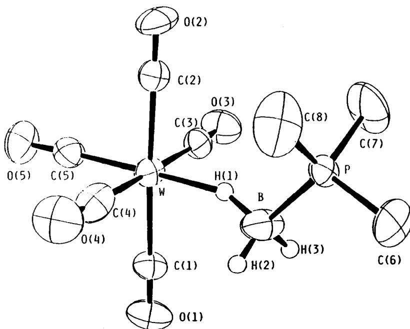
Fig. 11. ORTEP diagram of [W(CO)_5\{BH_3 \cdot P(CH_3)_3\}] [30].
