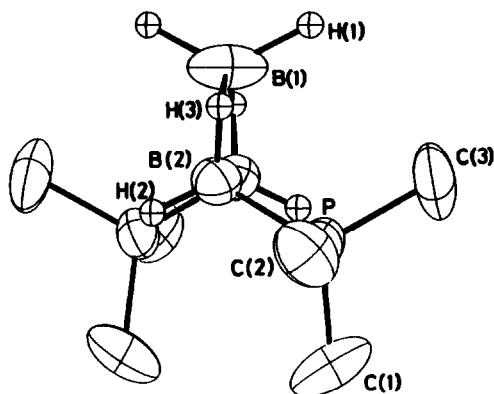
Fig. 4. The ORTEP plot of the structure of [\text{B}_3\text{H}_6 \cdot 2\text{P}(\text{CH}_3)_3]^+ cation (facing B–B axis) [24].
