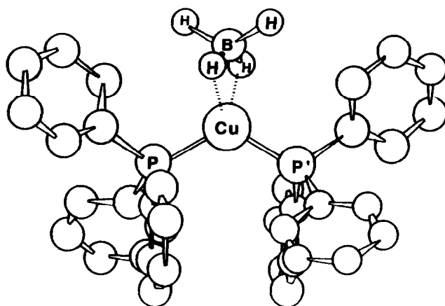
Fig. 1. Projection of borohydrido-bis(triphenylphosphine)copper(I) showing the molecular structure. Phenyl hydrogen atoms are not shown. (Modified from ref. 5).
